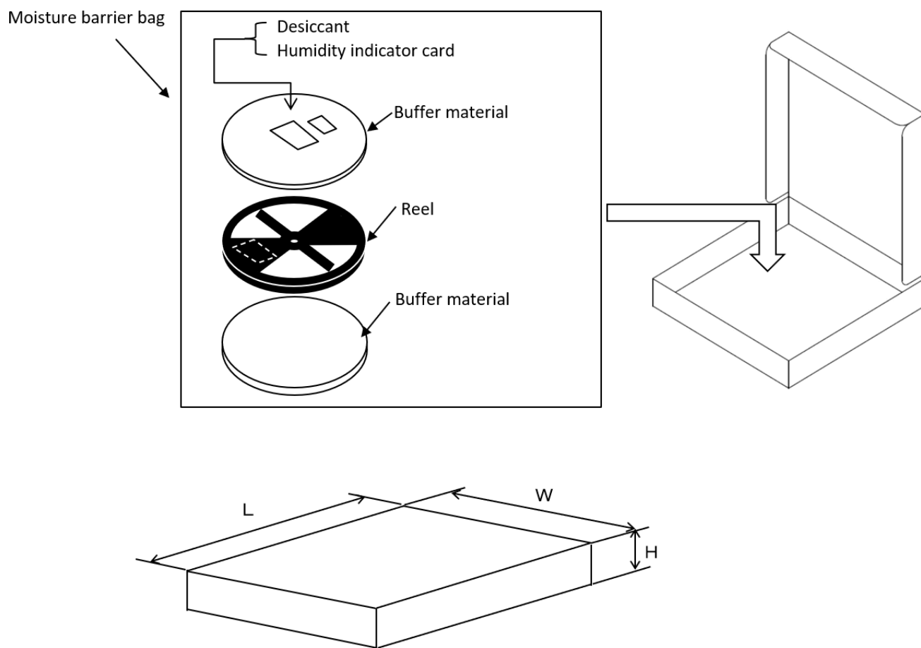
Figure 13-4 Packaging Detail
